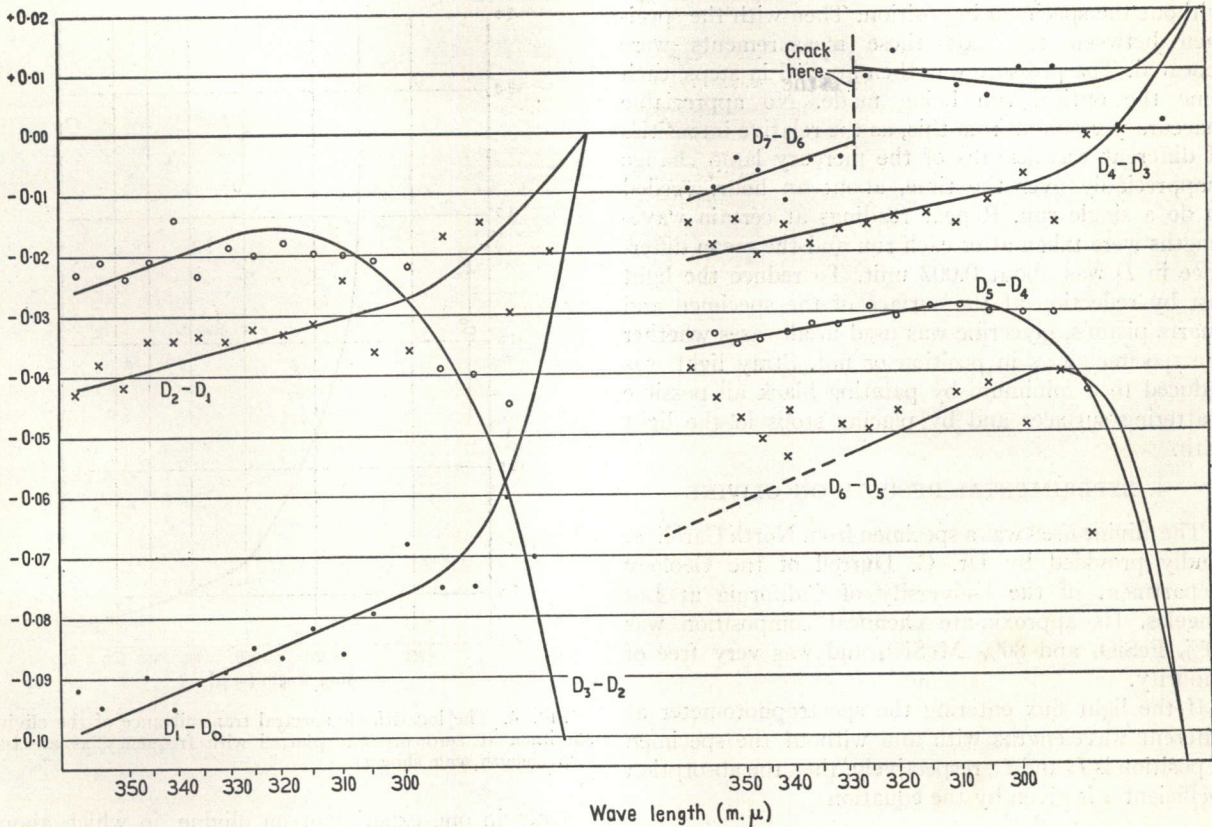
FIG. 2. The differences in the logarithmic spectral transmittances at successive pressures plotted against frequency (wavelength scale shown).
