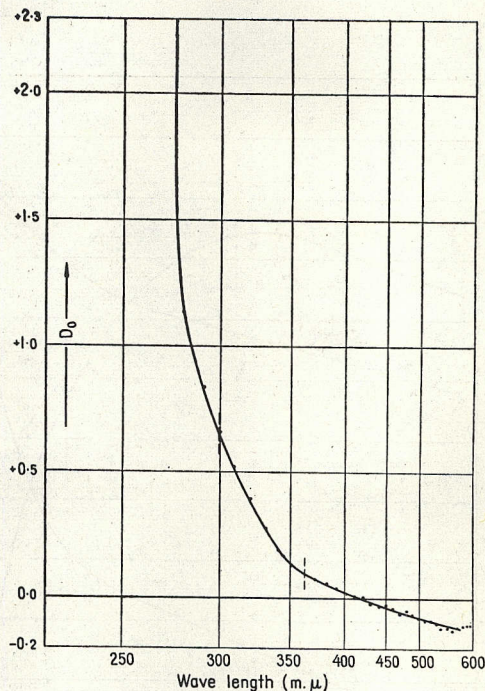
FIG. 4. The logarithmic spectral transmittance of the olivine specimen at zero pressure plotted with frequency as abscissa (wavelength scale shown).
