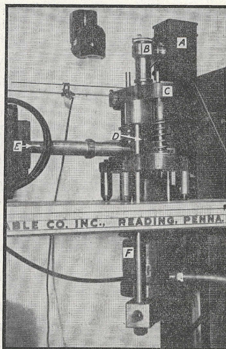
FIG. 1. High pressure apparatus.
