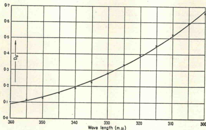
FIG. 5. Part of the curve of Fig. 4 fitted by a parabolic curve.
